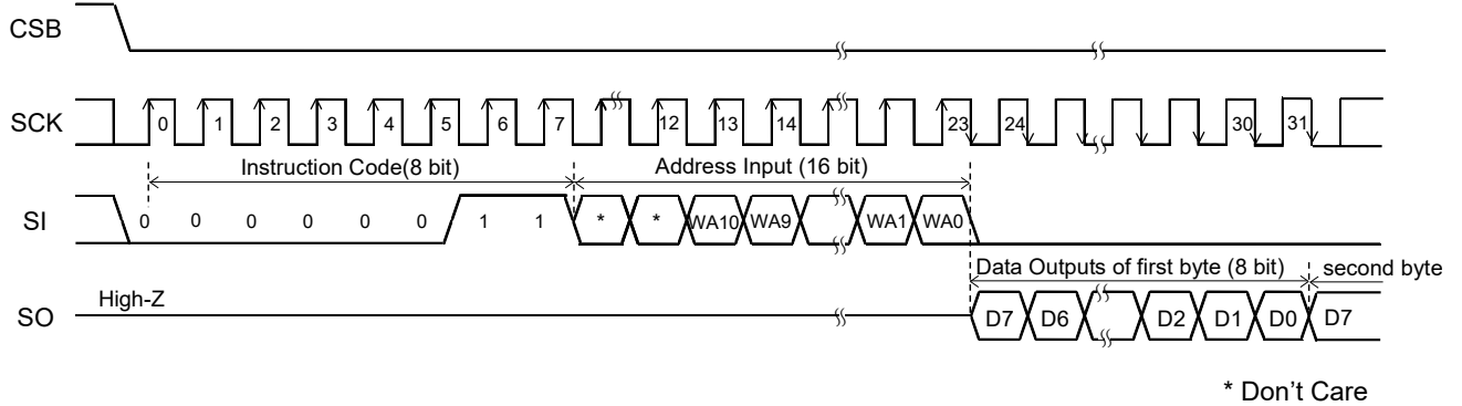
Figure 41. Read Command
