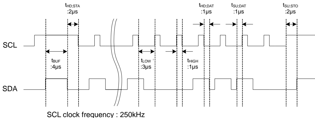
Figure 18. I 2 C Data Transmission Command Timing Diagram
