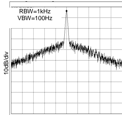
Figure 12. 24.6MHz Spectrum (V DD =3.3V, at C L =15pF)
