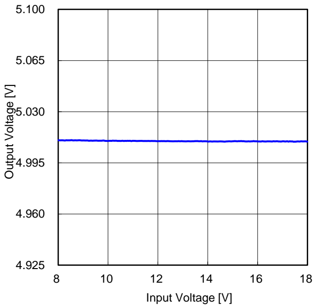
Figure 78. Line Regulation ( I_{OUT} = 3\ \text{A} )
