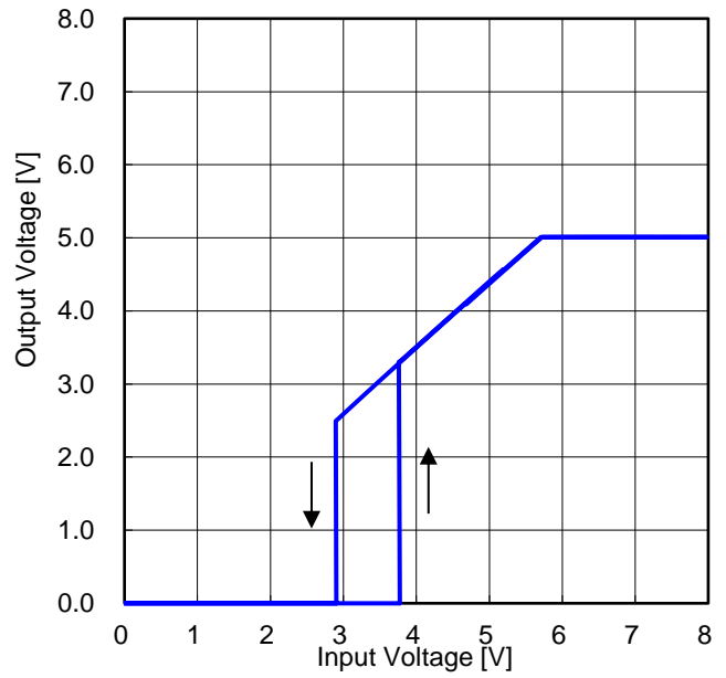
Figure 77. Output Voltage vs Input Voltage 2 ( R_{LOAD} = 1.66\ \Omega )
