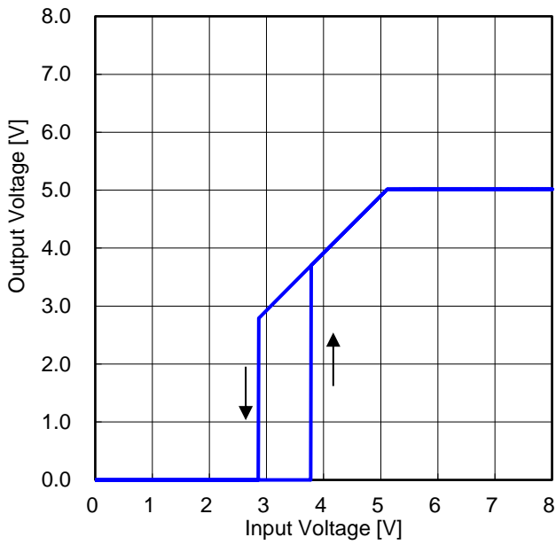
Figure 76. Output Voltage vs Input Voltage 1 ( R_{LOAD} = 166\ \Omega )
