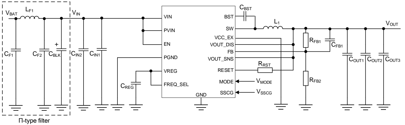
Figure 54. Reference Circuit 2
