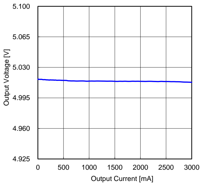
Figure 79. Load Regulation ( V_{IN} = 12\ \text{V} )
