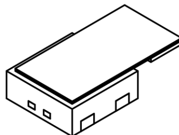
Figure 20. Sketch of the SHT4x with attached polyimide foil. 15
