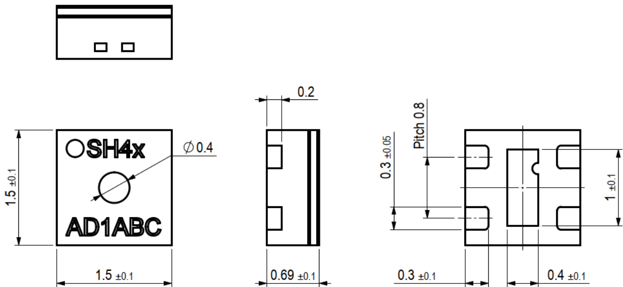
Figure 16. Dimensional drawing of SHT4xI with filter membrane including package tolerances (units mm)
