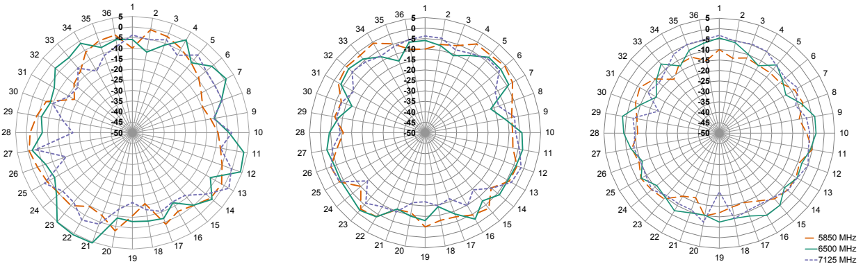
Figure 16. Radiation Patterns for ANT-W63WS3-SMA, Edge-Bent
