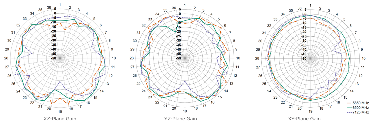
Figure 9. Radiation Patterns for ANT-W63WS3-SMA, Straight
