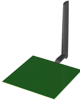
Figure 10. ANT-W63WS3-SMA on Edge of Ground Plane, Bent 90 Degrees (Edge-Bent)
