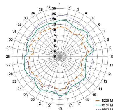
XY-Plane Gain
