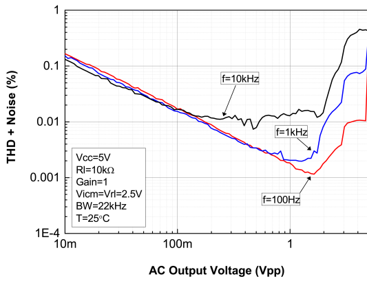
Figure 36. THD+N vs. output voltage
