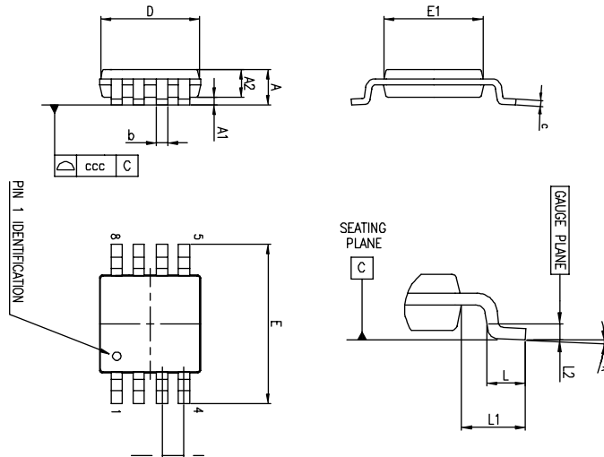
Figure 48. MiniSO8 package outline
