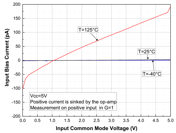
Figure 13. Input bias current vs. common-mode voltage at V_{\text{CC}} = 5\text{V}
