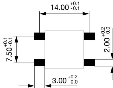
Gullwing Lead
