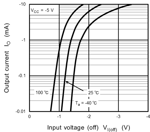
Fig. 7.2 I_O - V_{I(off)}
