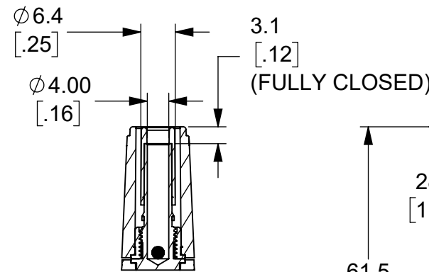
DETAIL B SCALE 2 : 1 (SOLDER TURRET)
