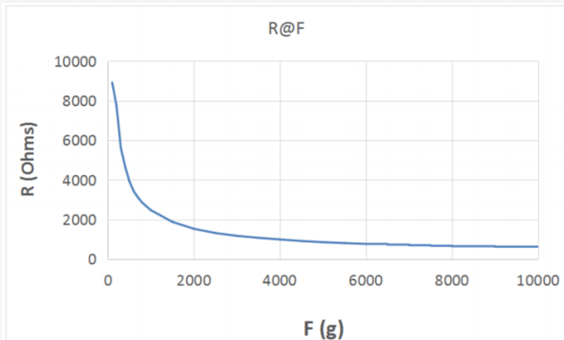
Force vs Resistance
