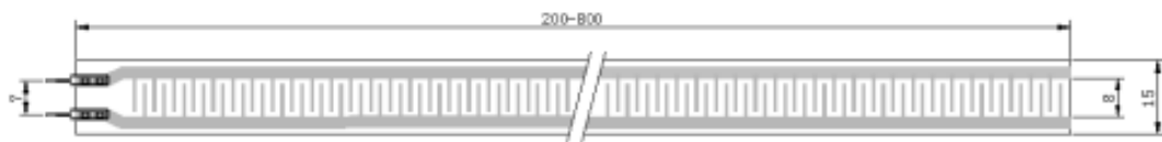
RP-L-170 Dimension Diagram
