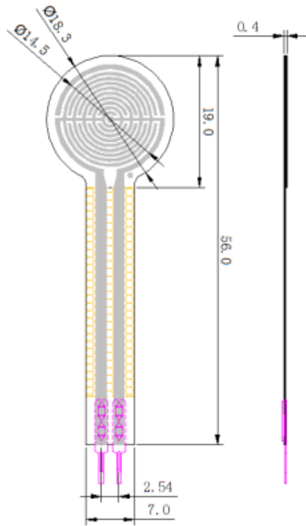
RP-C18.3-LT Dimension Diagram
