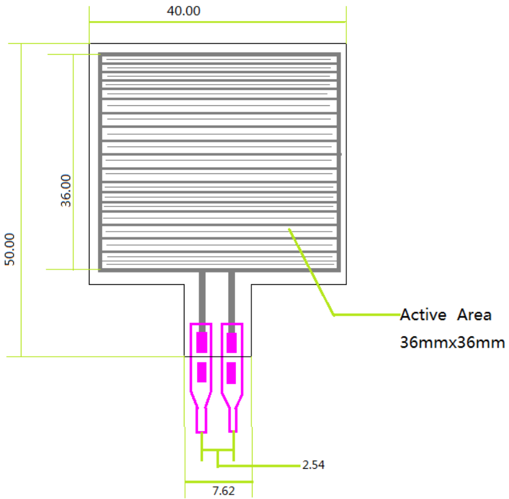
RP-S40-ST Dimension Diagram
