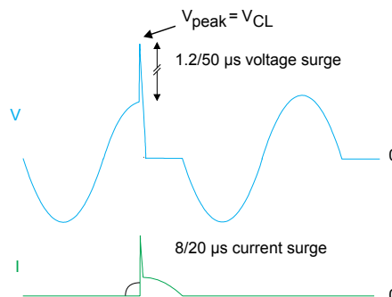
Figure 15. Typical voltage and current waveforms across the ACST1220H-8H during IEC61000-4-5 standard test
