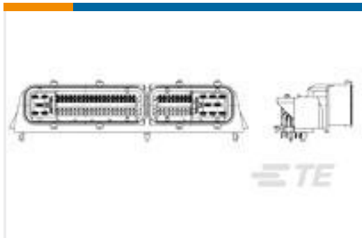
TE Part #1241434-1 121pos hybrid MQS .63 header 90deg
