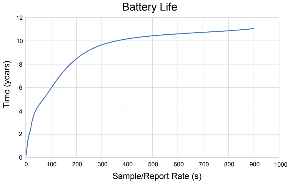
Battery life by sample/report rate (s)
