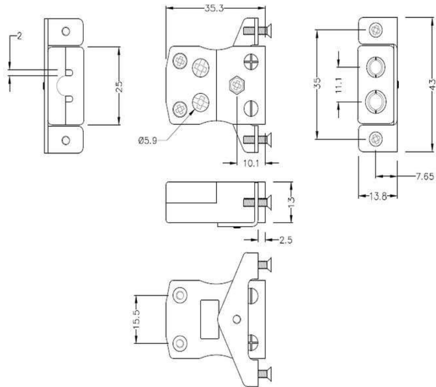
Standard Socket - Quick Wire with stainless steel mounting bracket
