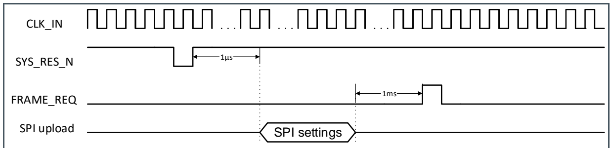
Figure 24: Reset Sequence When Changing Bit Mode
