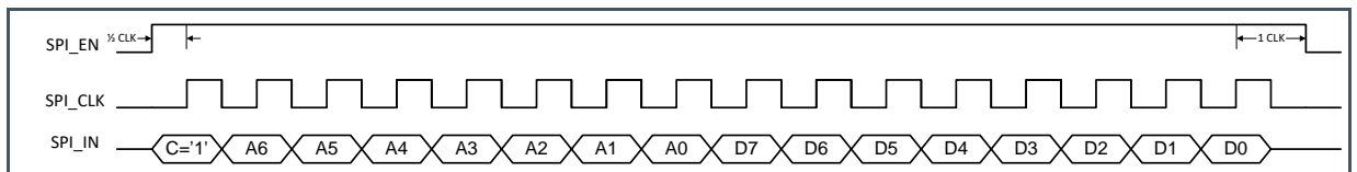
Figure 25: SPI Write Timing
