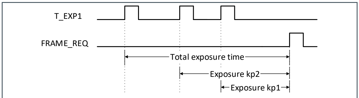
Figure 62: Timing of External Exposure Mode
