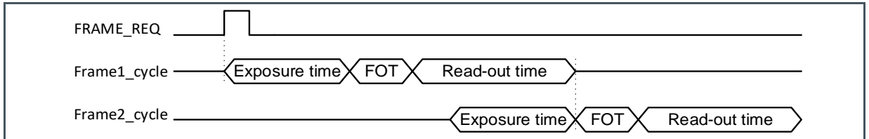
Figure 30: Request for 2 Frames in Internal Exposure Mode with Exposure Time < Read-Out Time
