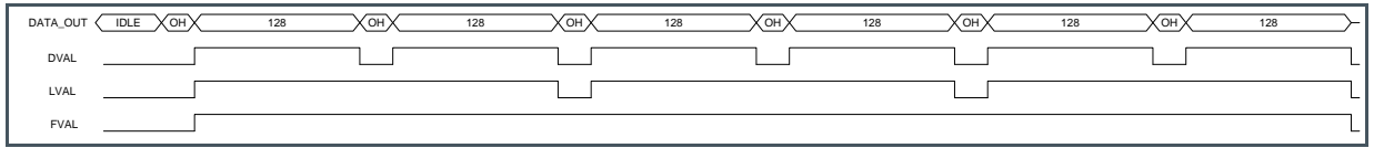
Figure 50: DVAL, LVAL and FVAL Timing in 8 Outputs Mode
