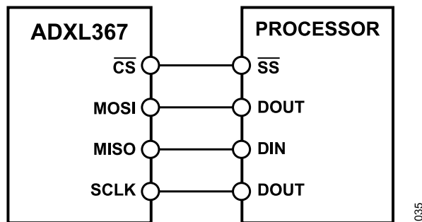
Figure 52. 4-Wire SPI Connection Diagram
