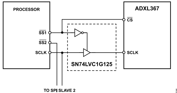
Figure 53. SCLK Protection Example
