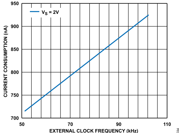
Figure 51. Current Consumption vs. External Clock Rate
