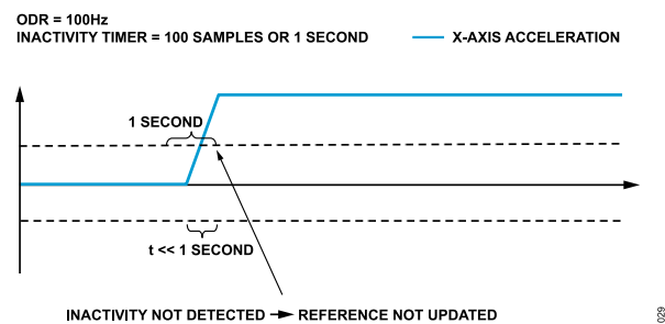
Figure 46. Referenced Inactivity Thresholds, Fast Change in Acceleration
