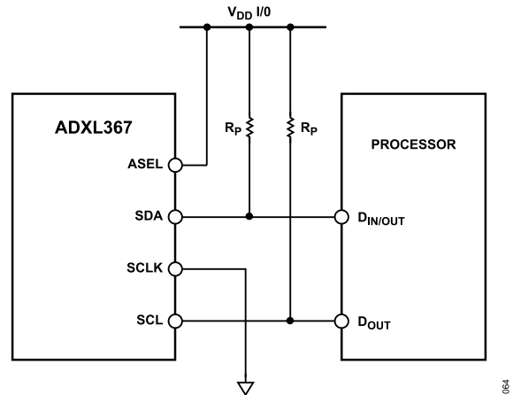
Figure 54. I 2 C Connection Diagram (Address 0x53)
