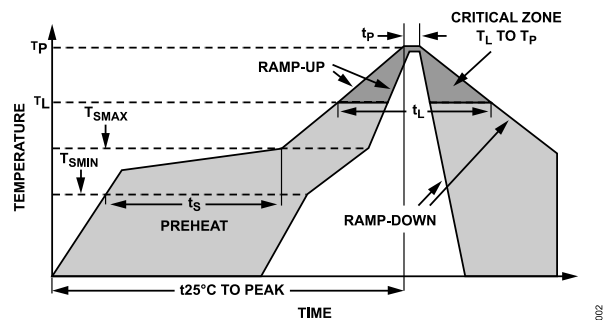
Figure 18. Recommended Soldering Profile
