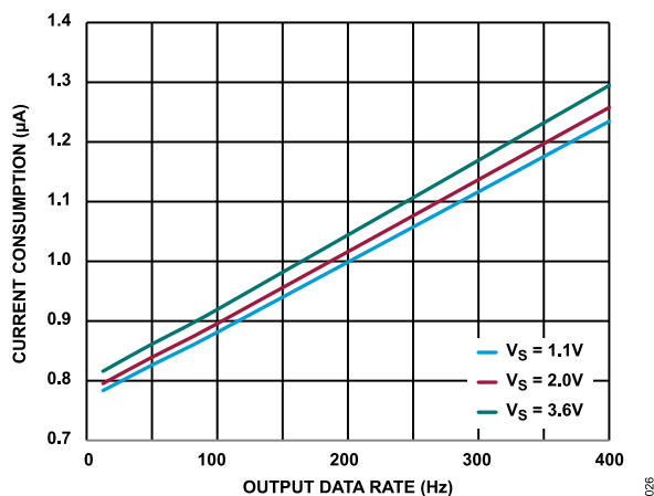
Figure 43. Current Consumption vs. Output Data Rate at Several Supply Voltages
