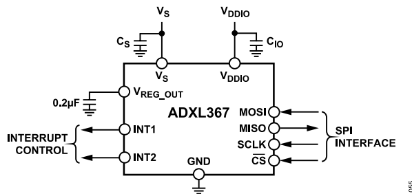
Figure 60. Recommended Bypass Capacitors
