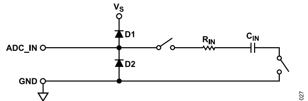
Figure 44. Equivalent Analog Input Circuit
