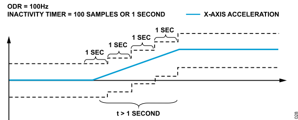
Figure 45. Referenced Inactivity Thresholds, Slow Change in Acceleration
