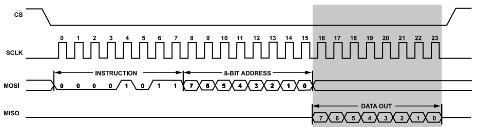
Figure 2. Register Read
