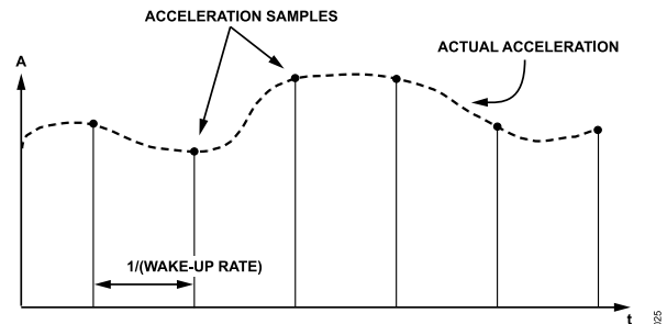
Figure 42. Acceleration Sampling
