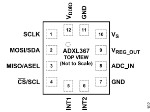
Figure 19. Pin Configuration
