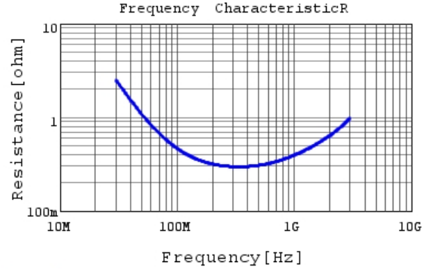
RDE5C2E100J1K1H03B R DC0V, 25degC
