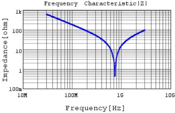
RDE5C2E100J1K1H03B |Z| DC0V, 25degC
