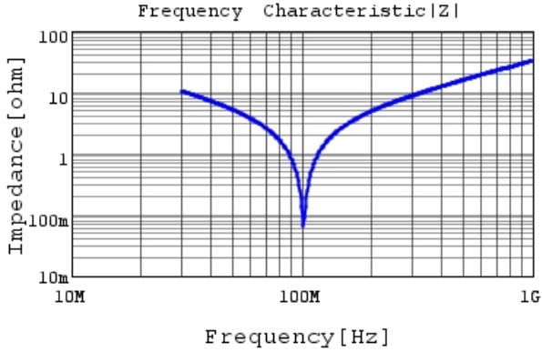
RCE5C2J471J1K1H03B |Z| DC0V,25degC
