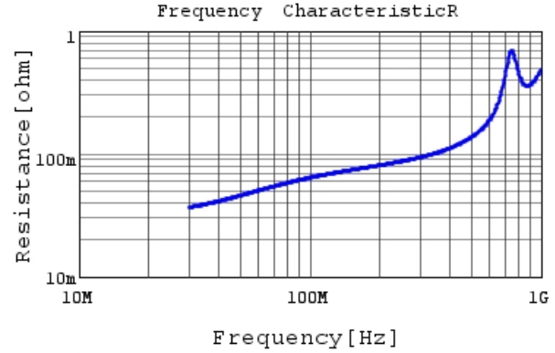
RCE5C2J471J1K1H03B R DC0V,25degC
