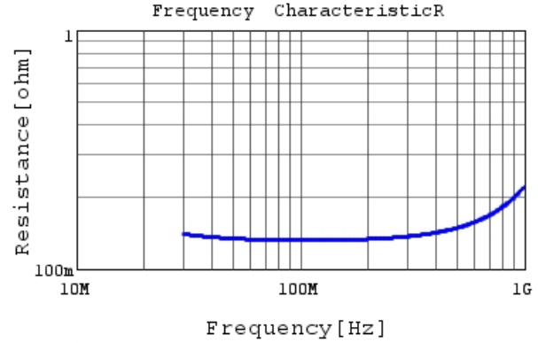
RCE5C2E151J1K1H03B R DC0V, 25degC
