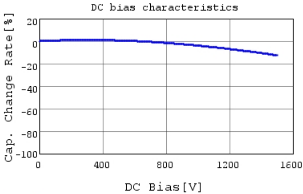
DE1B3RA331KN4AQ01F C-DC bias capchange, 20.0
