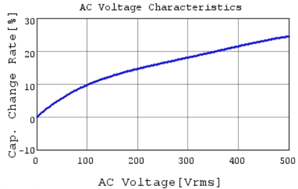
DE1B3RA331KN4AQ01F C-AC Voltage capchange, I
