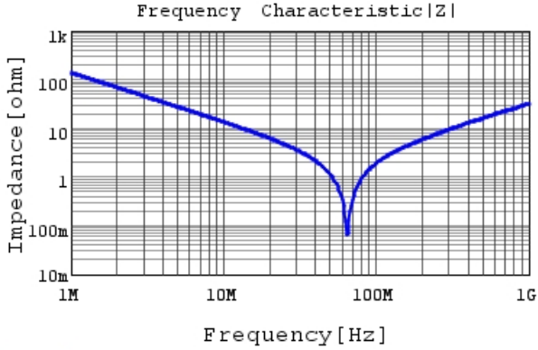
RCE5C2E122J1K1H03B |Z| DC0V, 25degC
