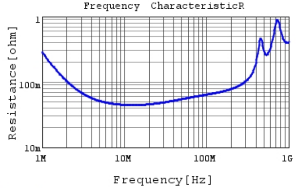
RCE5C2E122J1K1H03B R DC0V, 25degC
