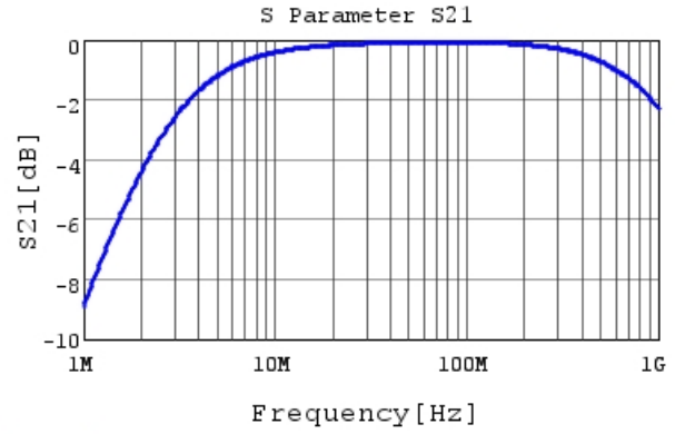
DE1B3RA681KN4AQ01F S21 DCOV, 20degC
