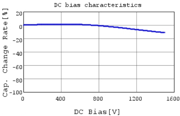
DE1B3RA681KN4AQ01F C-DC bias capchange, 20.0
