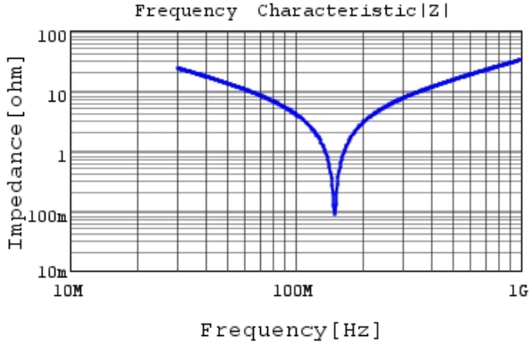
RDE5C2J221J1K1H03B |Z| DC0V, 25degC
