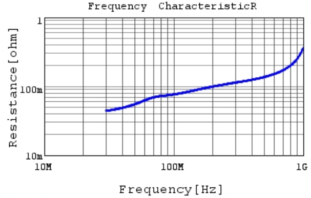
RDE5C2J221J1K1H03B R DC0V, 25degC
