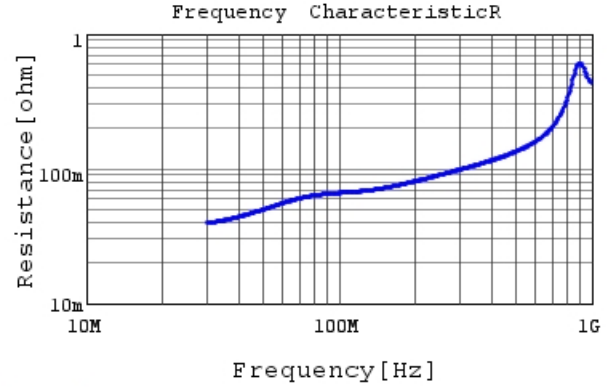
RCE5C2E391J1K1H03B R DC0V, 25degC
