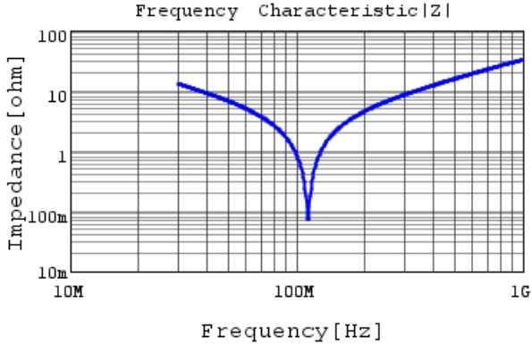
RCE5C2E391J1K1H03B |Z| DC0V, 25degC
