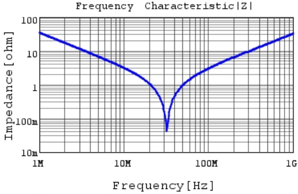
RCE5C2E472J1K1H03B |Z| DC0V, 25degC
