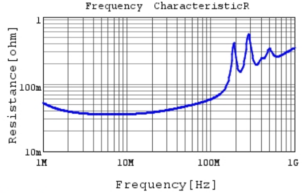
RCE5C2E472J1K1H03B R DC0V, 25degC
