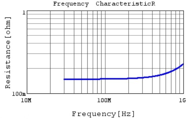
RCE5C2E121J1K1H03B R DC0V, 25degC
