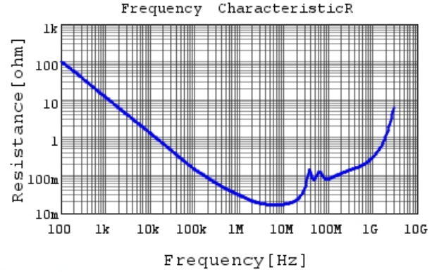
GRM43DR72J104KW01 R DCOV, 25degC
