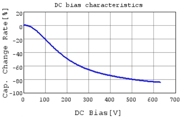
GRM43DR72J104KW01 C-DC bias capchange, 25.0c
