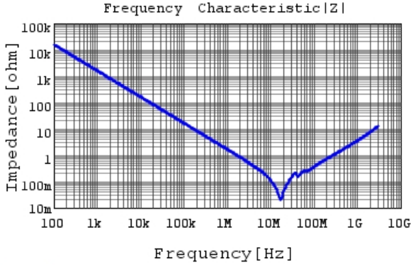
GRM43DR72J104KW01 |Z| DCOV, 25degC
