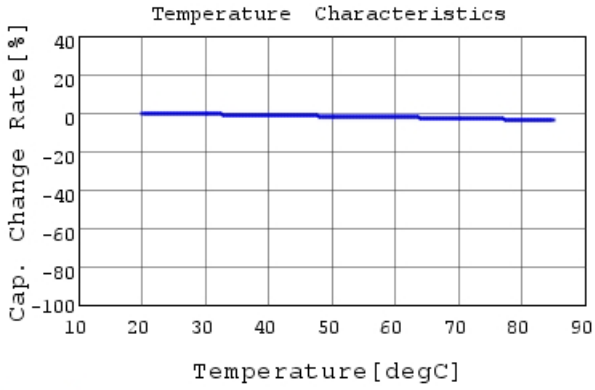
DE21XSA470KN2AT01F C-Temp. capchange, DCOV,
