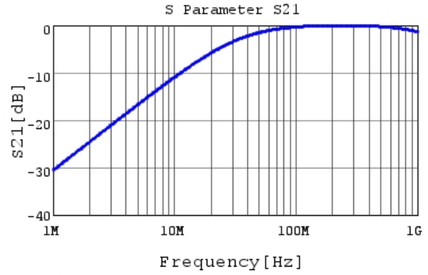
DE21XSA470KN2AT01F S21 DCOV, 20degC
