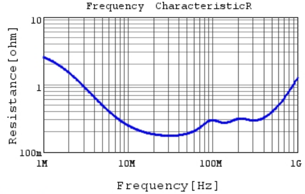
DE21XSA470KN2AT01F R DCOV, 20degC
