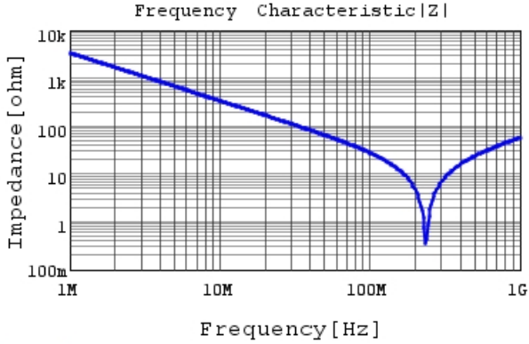
DE21XSA470KN2AT01F |Z| DCOV, 20degC
