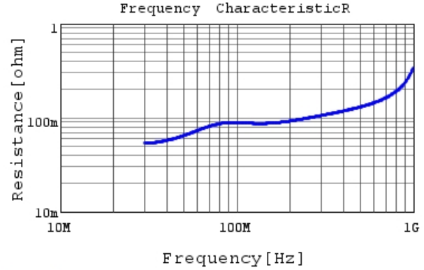
RCE5C2E221J1K1H03B R DC0V, 25degC
