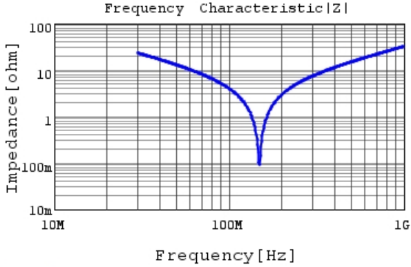
RCE5C2E221J1K1H03B |Z| DC0V, 25degC
