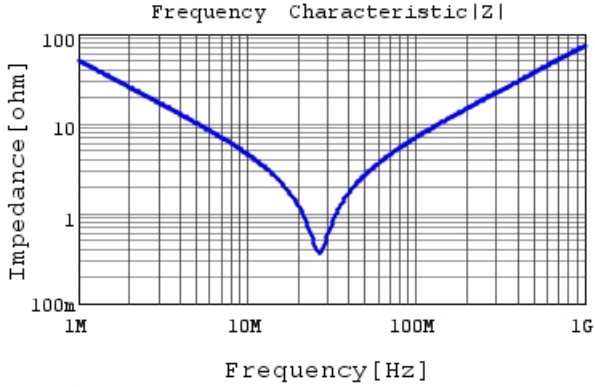
DE1E3RA332MN4AH01F |Z| DCOV, 20degC
