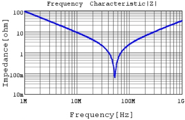
RCE5C2E182J1K1H03B |Z| DC0V, 25degC
