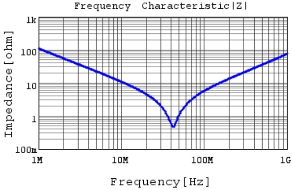
DE2E3SA152MN3AX02F |Z| DCOV, 20degC
