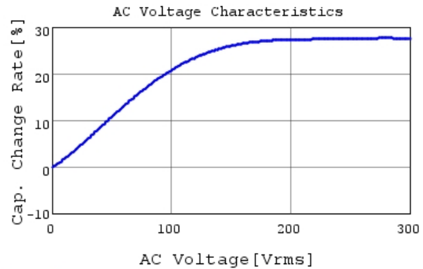
DE2E3SA152MN3AX02F C-AC Voltage capchange, I
