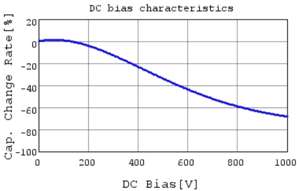
DE2E3SA152MN3AX02F C-DC bias capchange, 20.0
