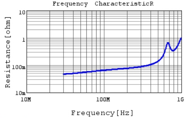
RCE5C2J561J1K1H03B R DC0V, 25degC
