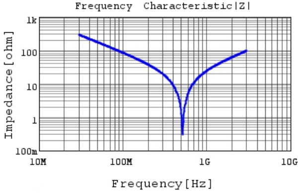
RDE5C2E180J1K1H03B |Z| DC0V, 25degC
