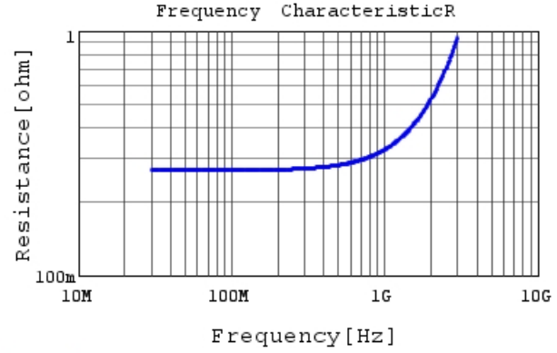
RDE5C2E180J1K1H03B R DC0V, 25degC
