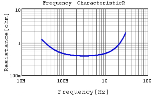
RDE5C3A100J2K1H03B R DC0V, 25degC
