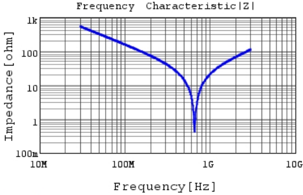
RDE5C3A100J2K1H03B |Z| DC0V, 25degC
