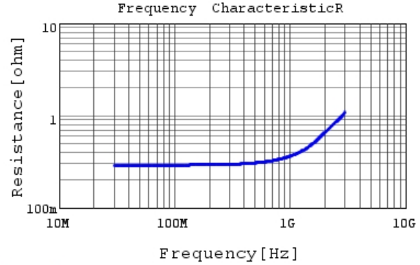
RDE5C2E330J1K1H03B R DC0V, 25degC
