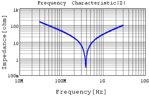
RDE5C2E330J1K1H03B |Z| DC0V, 25degC
