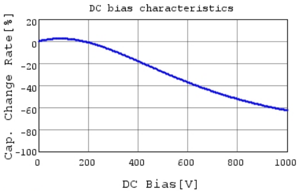
DE2E3SA472MJ3BT02F C-DC bias capchange, 20.0
