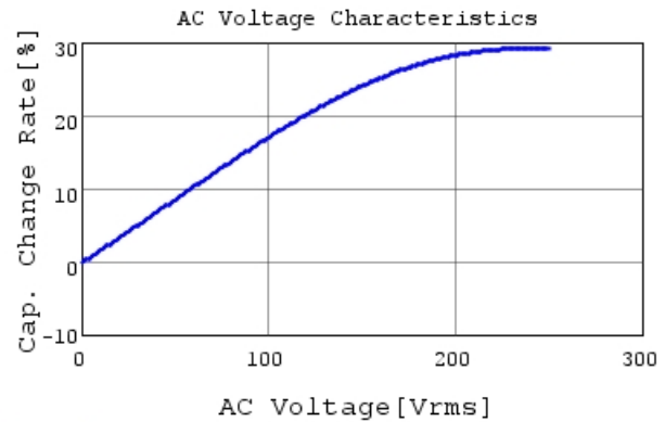
DE2E3SA472MJ3BT02F C-AC Voltage capchange, I
