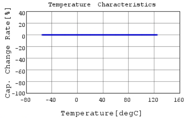
RCE5C2E330J1K1H03B C-Temp. capchange, DC0V,
