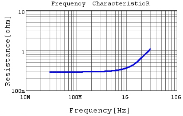
RCE5C2E330J1K1H03B R DC0V, 25degC
