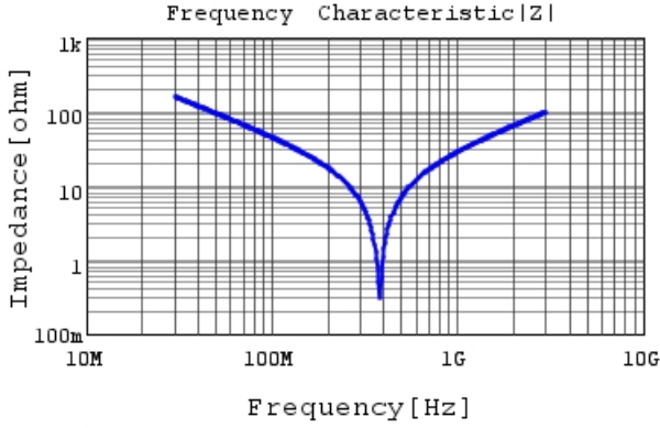
RCE5C2E330J1K1H03B |Z| DC0V, 25degC
