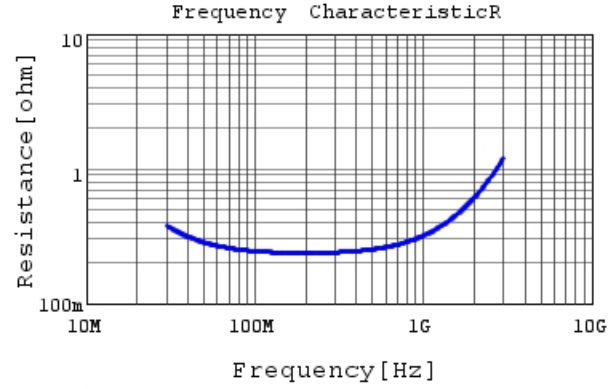
RCE5C2E390J1K1H03B R DC0V, 25degC
