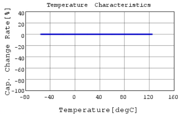
RCE5C2E390J1K1H03B C-Temp. capchange, DC0V,
