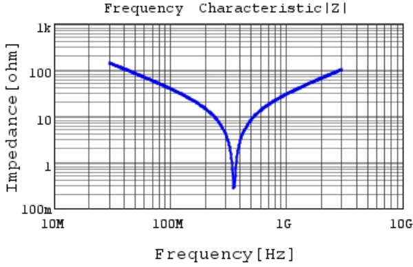
RCE5C2E390J1K1H03B |Z| DC0V, 25degC
