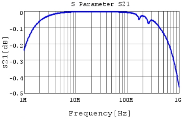
RCE5C2E682J1K1H03B S21 DC0V, 25degC
