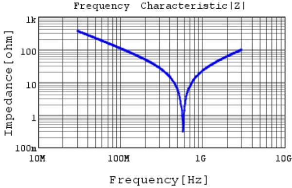
RCE5C2J150J1K1H03B |Z| DC0V, 25degC
