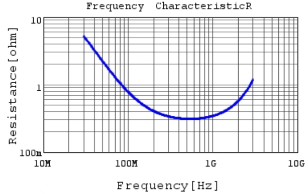
RCE5C2J150J1K1H03B R DC0V, 25degC
