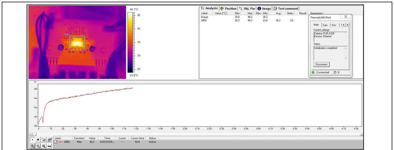
Figure 9 Peak power P_{out} = 103 W with 6 \Omega load \pm 32 V
