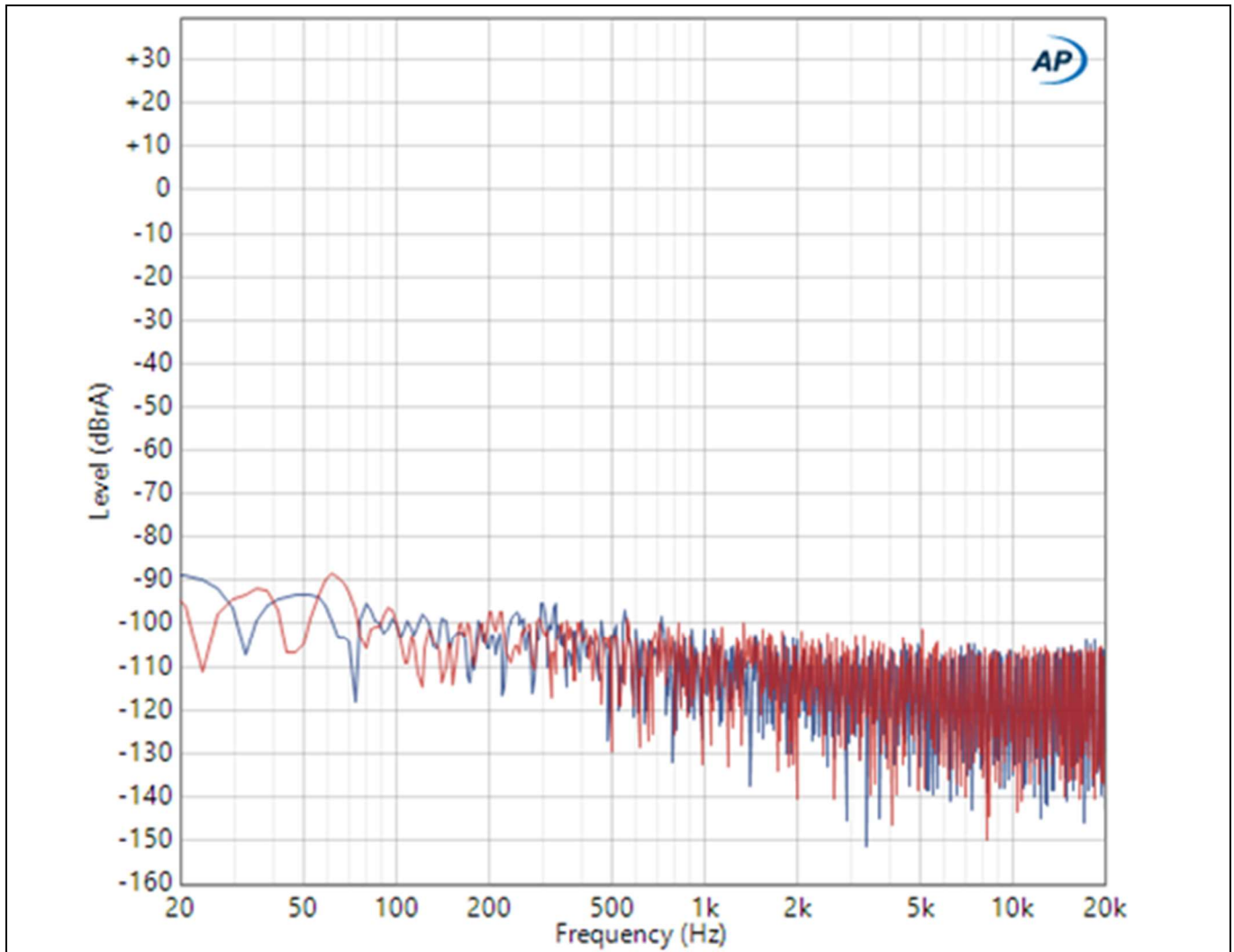
Figure 6 Noise floor 2\ \Omega load
