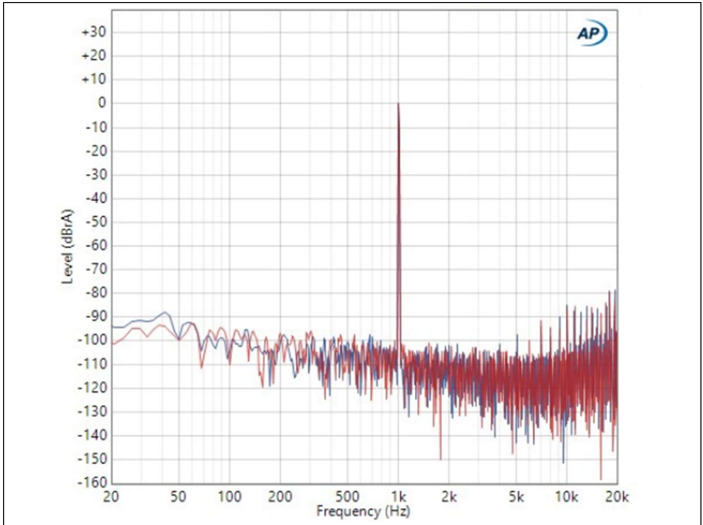
Figure 7 Noise floor with 1 V RMS output 2 Ω load
