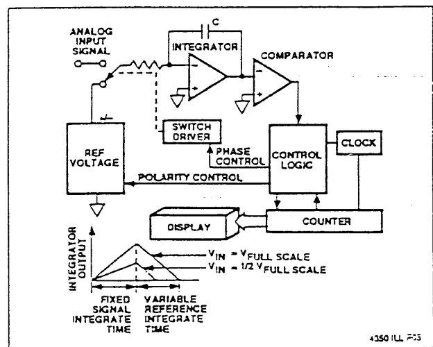
Figure 3A Basic Dual Slope Converter
