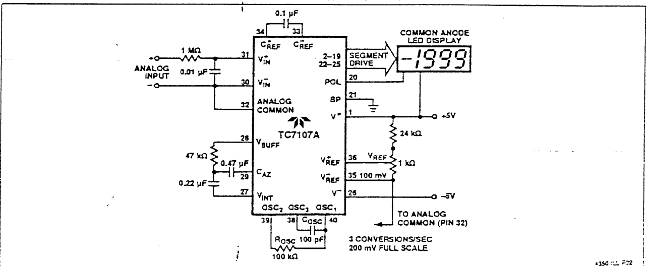
Figure 2 TC7107A Typical Operating Circuit
