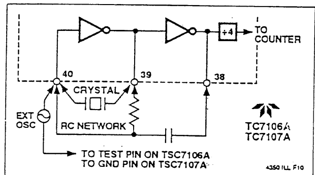
Figure 8 Clock Circuits
