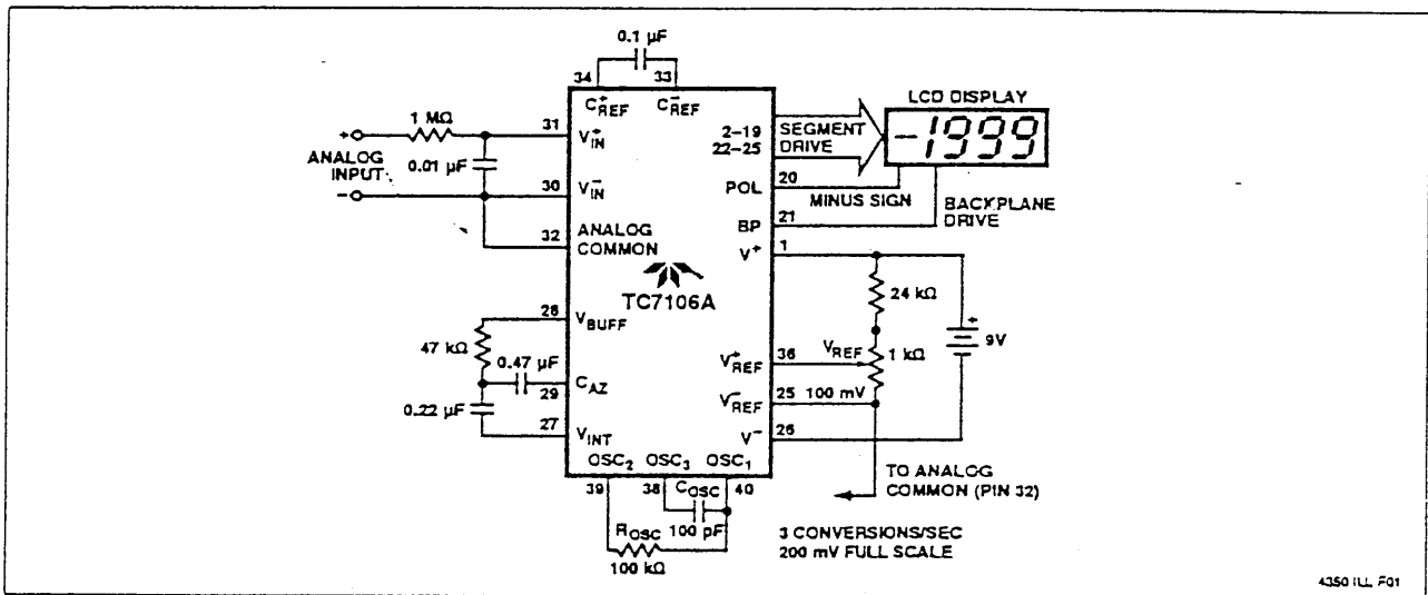
Figure 1 TC7106A Typical Operating Circuit
