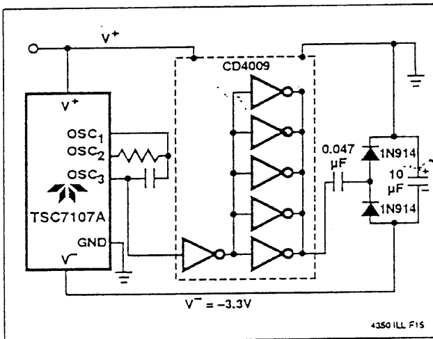
Figure 14 Generating Negative Supply From +5 V
