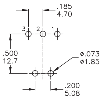
P.C. MOUNTING
