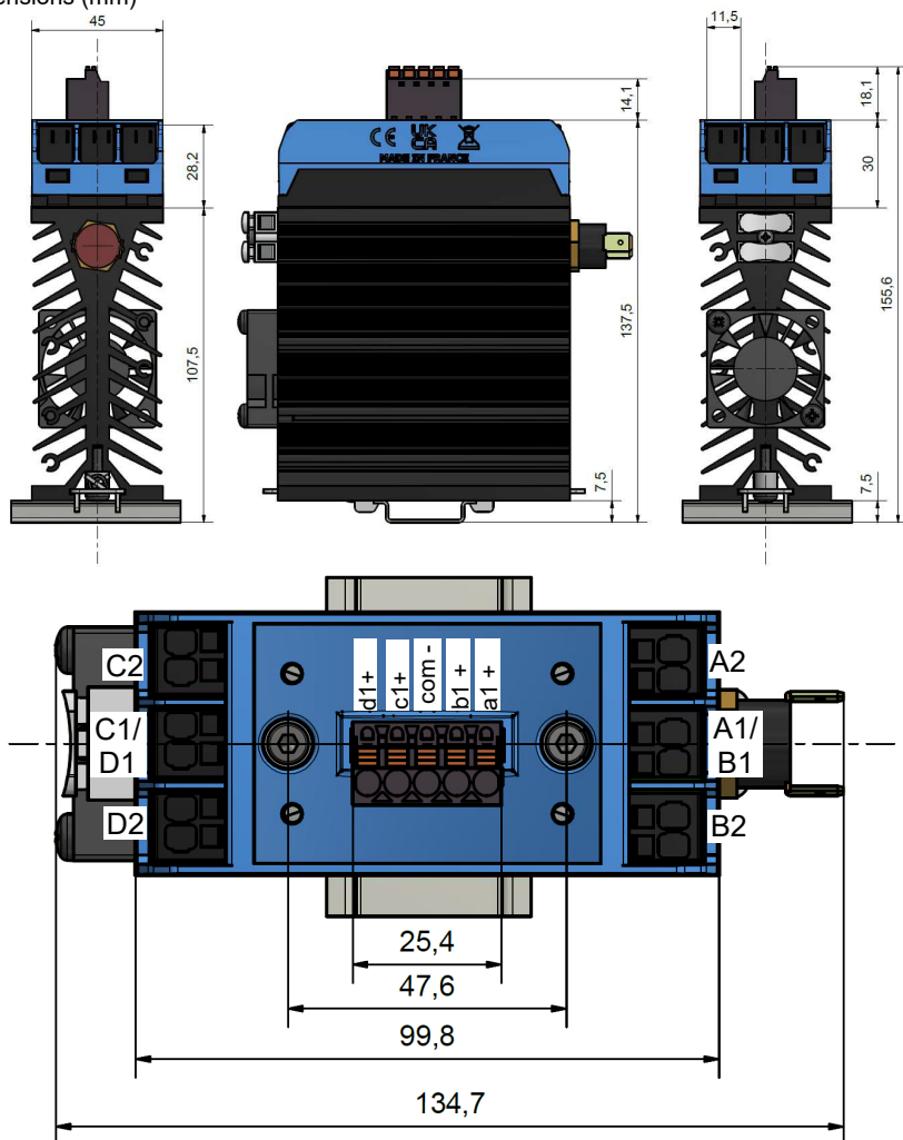
Dimensions (mm)
