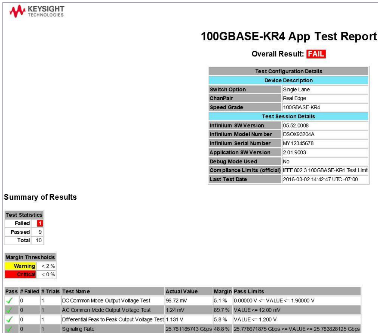
Figure 5. The D9010BJBC 100GBASE-KR4 compliance test application software results screen shows a summary of the tests performed, pass/fail status, and margin. Clicking on a specific test also shows the test specification and a measurement waveform, if appropriate.
